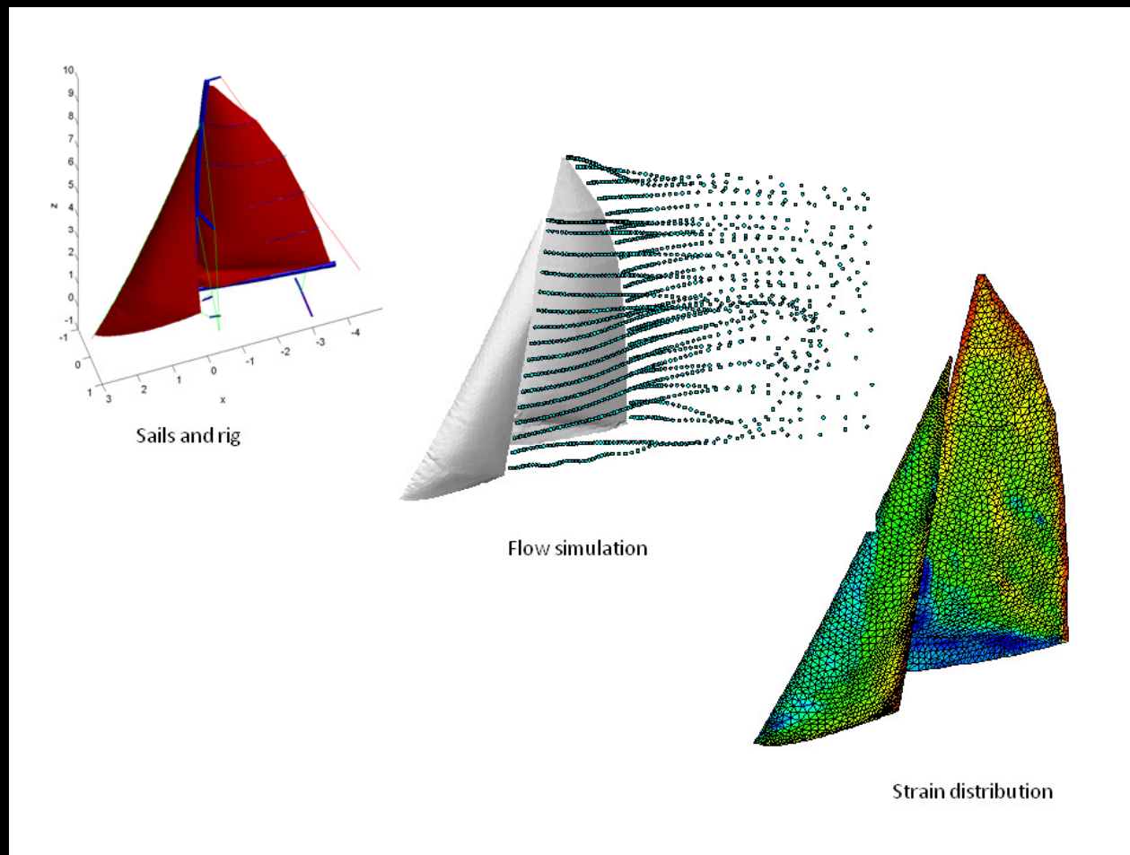
FSI simulation of the complete J80 rigging and sails
